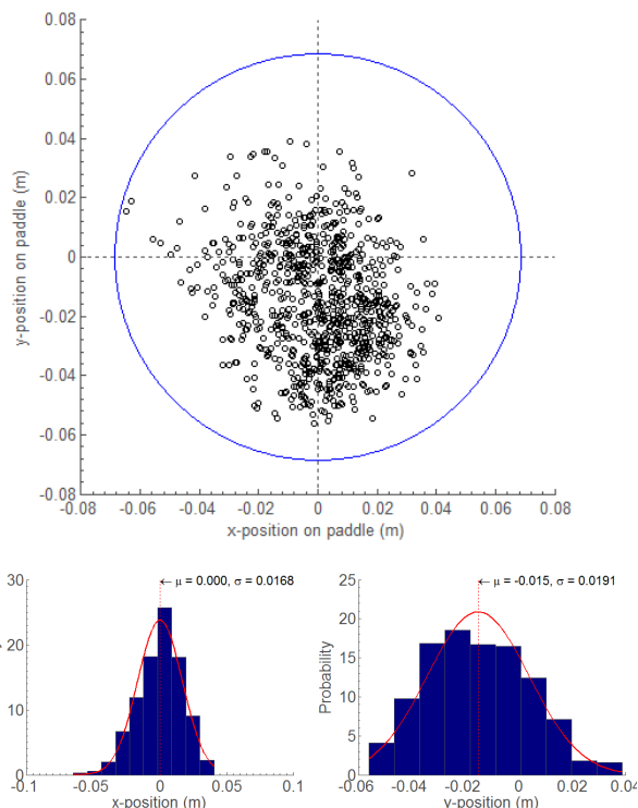
Fig. 7. Contact locations between ball and paddle relative to the center of the paddle. Top: x- and y-positions on the paddle; blue circle approximately shows the paddle size (0.15m in diameter). Bottom: Fitted contact coordinate distributions for x- and y-positions. Contact positions are calculated as the difference between positions of the ball and the center of the paddle. The effect of the discretization (the actual point of contact being somewhere between the measurements) is ignored in this case; we used coordinates from the lowest (in z) measurement.
