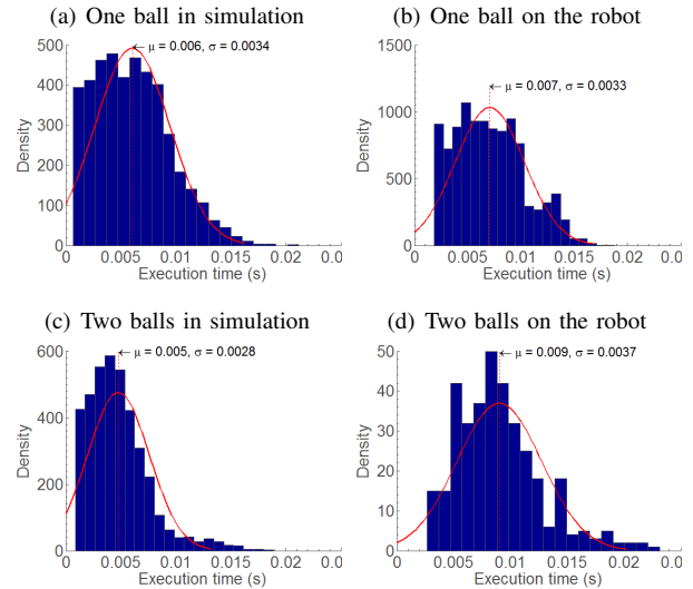
Fig. 1. Execution time histograms and fit Gaussians for one and two ball juggling in simulation and on the real robot.
